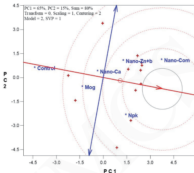
Fig. 5. Ideal entry view of treatment by trait (TT) biplot, showing the relationships of different nano, bio and bulk fertilizer treatments with ideal entry (treatment) in potato. For traits' abbreviations, refer to the text
