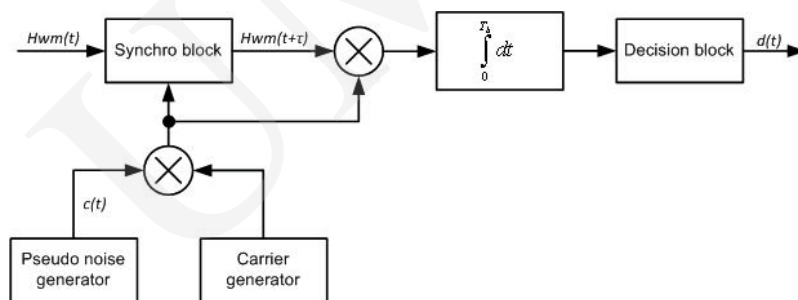
Fig. 6. Schematic diagram for the watermark extractor.
