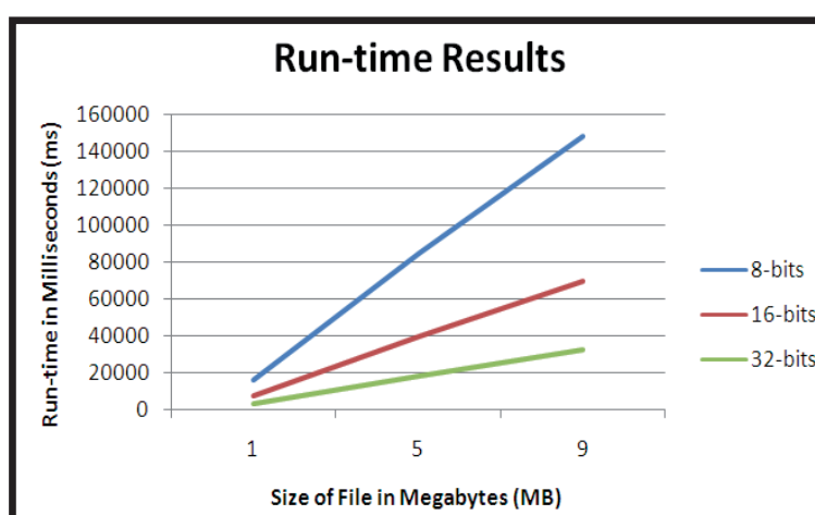
Fig. 2. Comparison of run-time results m = 8, 16 and 32 .
