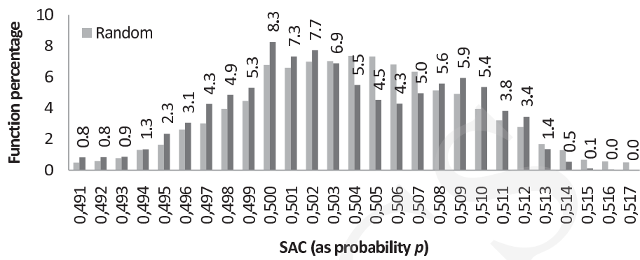
Fig. 10. SAC of S-boxes with removed affine equivalence.
