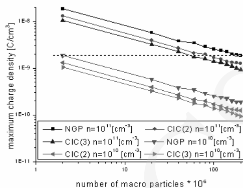
Fig. 9. Comparison of maximum deviations of charge density averaged over five middle grid layers for the two plasma concentration values ( 10^{10} [cm ^{-3} ] and 10^{11} [cm ^{-3} ])
