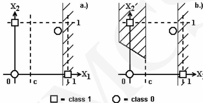
Fig. 2. Subsequent stages of an evolution of decision space for single Sigma-if neuron with two neuronal inputs during signals aggregation, a) division into two problems and solving of a linear problem, b) connection of decision spaces of the first and second stages
