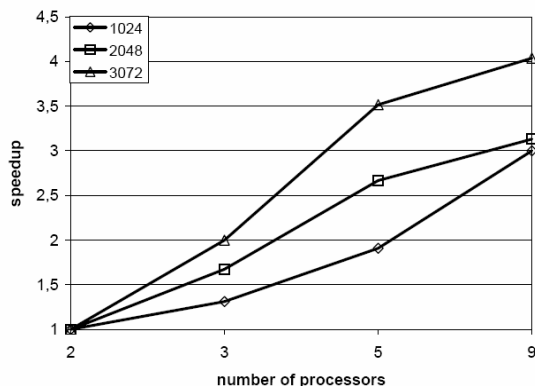
Fig. 2. SGI Power Challenge; speedup of Kruskal algorithm for the graphs of sizes 1024, 2048, 3072
