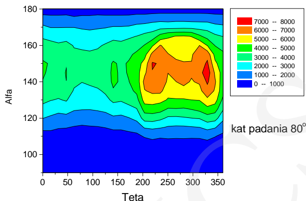
Fig. 2. Contour plots (lines of equal intensity) of the angular distribution of scattered particles for N->Ti (1500eV) and angle of incident \phi=80^{\circ}
