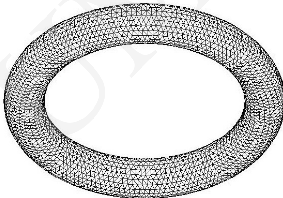
Fig. 5. Unstructured mesh on a torus – coarse mesh
