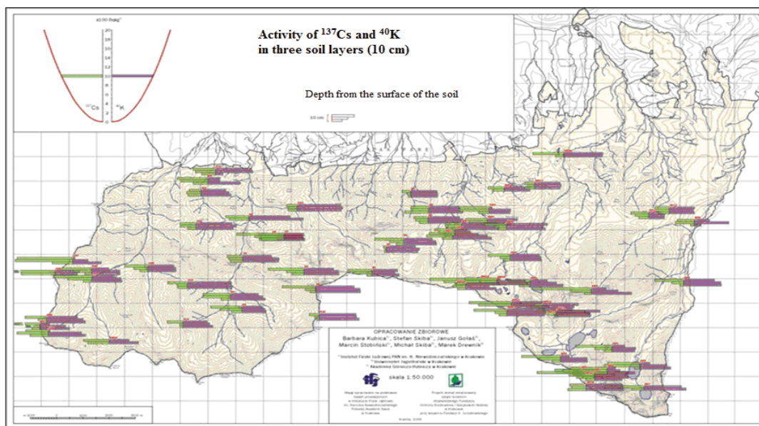
Fig. 1. The map of the Tatra National Park, taking into account the radioactivity of ^{137}\text{Cs} and ^{40}\text{K} expressed in Bq/kg in soil samples
