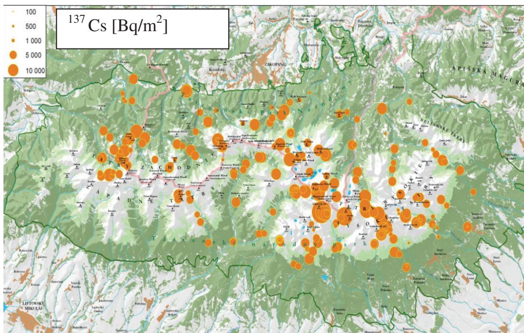
Fig. 3. Changes of the activity of ^{137}\text{Cs} [ \text{Bq}/\text{m}^2 ] in the surface layer of soil in the Tatra mountains.
